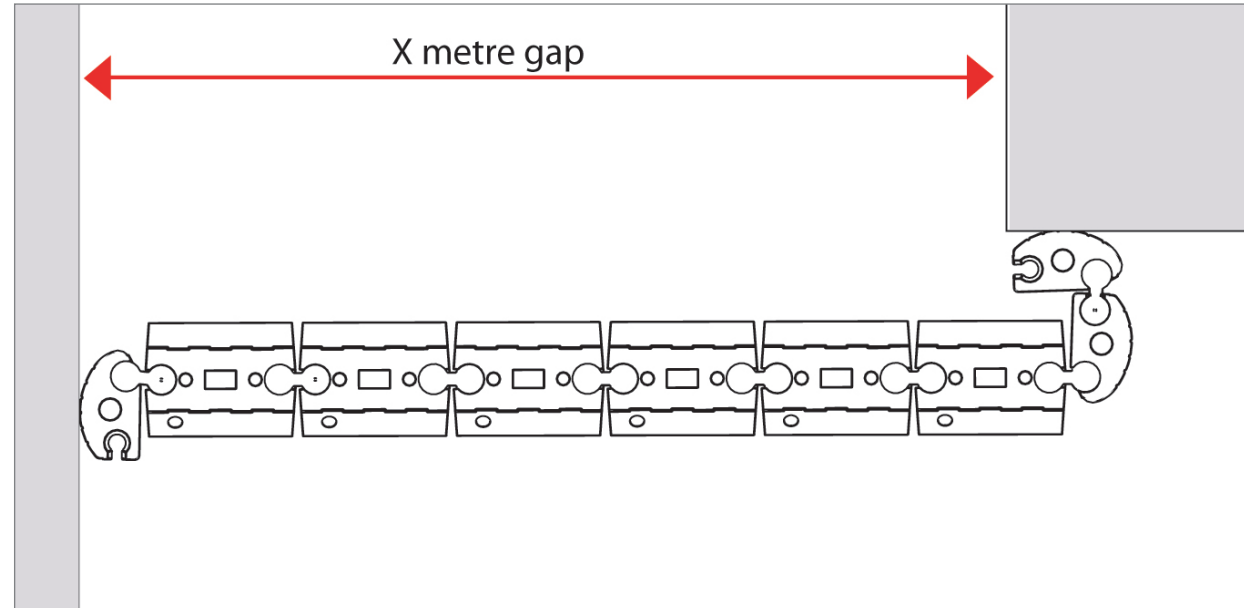
Flood Barrier 900mm CAD Diagram
